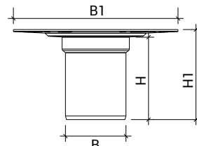
STC-DC100ABS B1 = 300 mm H = 150 mm H1 = 163,5 mm
