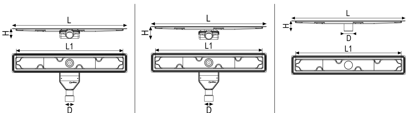
STL-BL DRAIN LOW: H = 56 mm D = 50 mm
