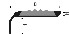
Aluminum - Brass H1 = 5 mm SM14: H = 14 mm SM28: H = 28 mm
