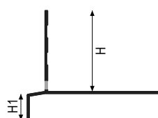
BD - Aluminum (with draining holes) H1 = 18 mm
