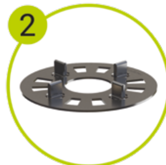
SUPATRAYTAB2 and SUPATRAYTAB4 for 2mm 4mm joints
