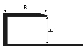
Aluminum B = 15 mm
