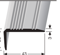
225 U/FW ungebohrt undrilled non percé
