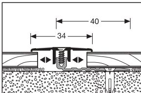
388 AS \updownarrow 5 - 11,5 mm*
