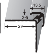
153 U ∅ 3 - 5 mm ungebohrt undrilled non percé
