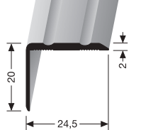
235 U/FW ungebohrt undrilled non percé
