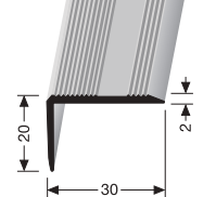
227 U/FW ungebohrt undrilled non percé
