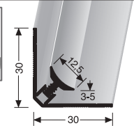
163 U ∅ 3 - 5 mm ungebohrt undrilled non percé
