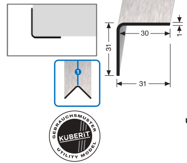
143 U ungebohrt undrilled non percé
