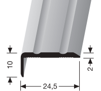
236 U/FW ungebohrt undrilled non percé
