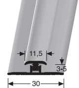
179 U ∅ 3 - 5 mm ungebohrt undrilled non percé
