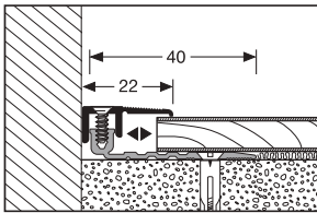
387 AS \updownarrow 5 - 11,5 mm*
